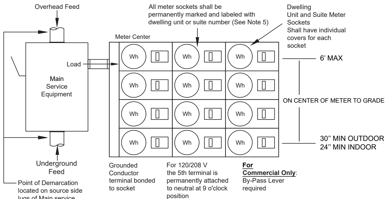
FIGURE 1: MULTIPLE METER / DISCONNECT UNITS
